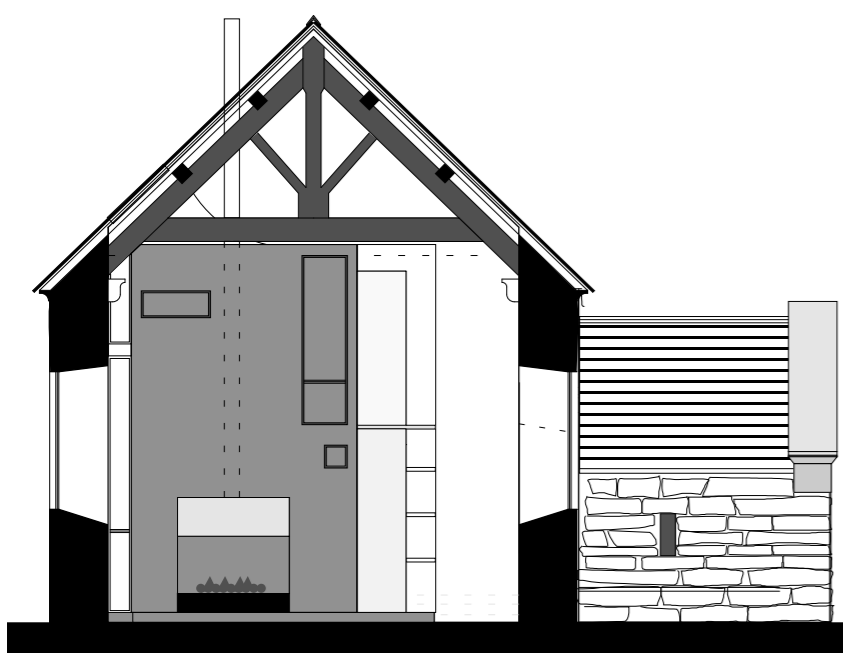
Section E-E
