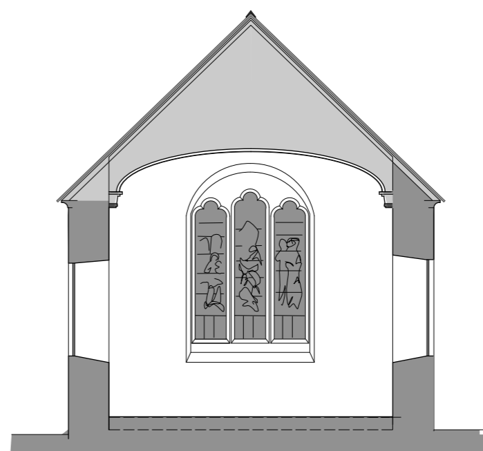
Section G-G
