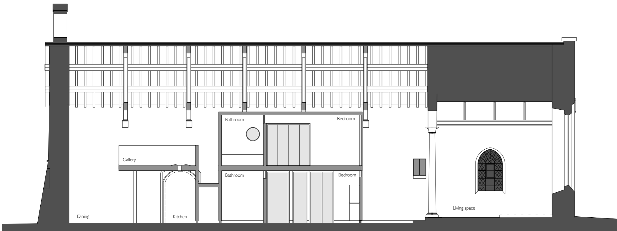
Section H-H
